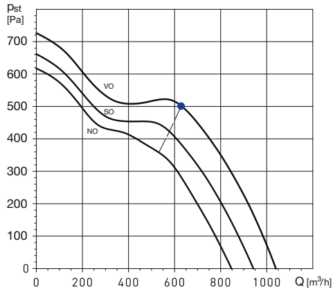
TDx2-1300/250
