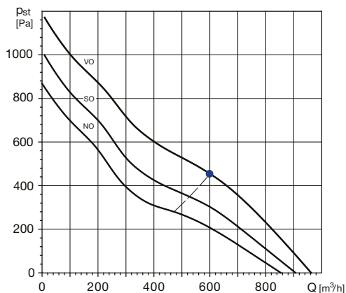
TDx2-1000/250
