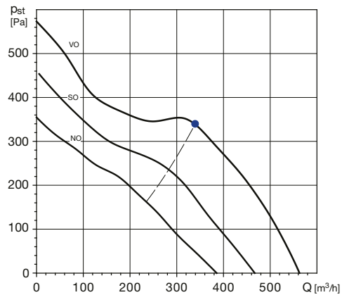
TDx2-500/150, TDx2-500/160
