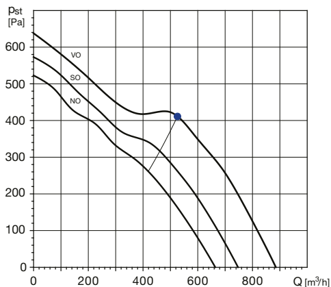
TDx2-1000/250
