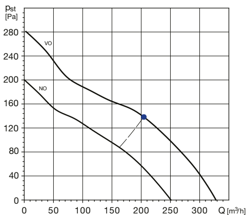
TDx2-350/125
